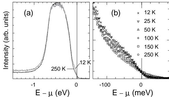
Figure 5: T dependent angle integrated PES data for \text{Li}_{0.9}\text{Mo}_6\text{O}_{17} , measured at h\nu = 33 eV, \Delta E = 30 meV, \Delta\theta = \pm 6^\circ .
